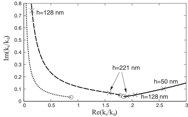
FIG. 7. Trajectory in the complex plane of the quantity \frac{k_x}{k_0} for three different waveguided modes (solid line: first even mode; dashed line: first odd mode; dotted line: second even mode) when the width of the metal goes from 380 nm (circles) to 10 nm. The permittivity of the metal is taken equal to the permittivity of gold at 608 nm, \epsilon \simeq -10.01 + 1.44i . Intermediate thicknesses of 221 nm (when the real part of the index of the odd mode becomes smaller than 1.58, so that the coupled plasmon picture becomes less relevant), 128 nm (when the odd mode can be considered nonpropagative, and the coupled plasmon picture is not relevant any more), and 50 nm are indicated on the curves.
