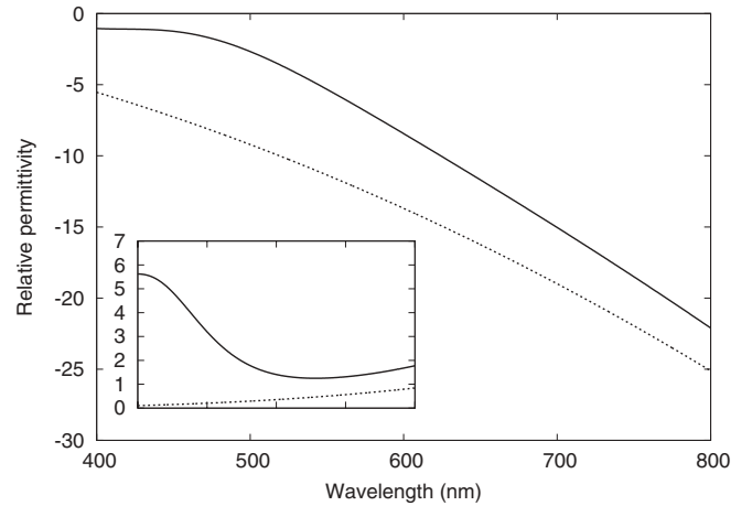
FIG. 1. Real part of the relative permittivity of gold in the visible (solid line) and Drude permittivity according to Ref. 39 (dotted line). The difference is the contribution of bound electrons. Inset: Imaginary part of the relative permittivity, same x scale, same lines.
