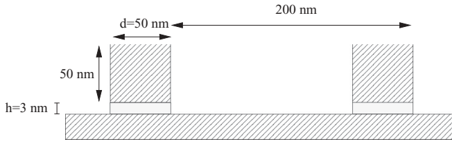
FIG. 10. Strips (rods with a 50 \text{ nm} \times 50 \text{ nm} section) are separated from the metallic film by a 3 \text{ nm} thick dielectric with an optical index of 1.58 . The structure considered here is periodic, with a 200 \text{ nm} period.
