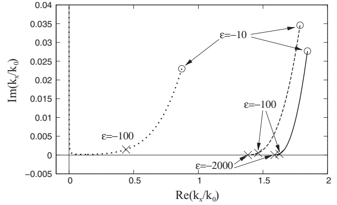
FIG. 6. Trajectory in the complex plane of the quantity \frac{k_x}{k_0} for three different waveguided modes (solid line: first even mode; dashed line: first odd mode; dotted line: second even mode) when the permittivity of the metal goes from \epsilon = -10 + i (circles) to \epsilon = -2000 + i , for a thickness of the waveguide of 500 nm and a dielectric with a 1.58 optical index. The intermediate value of -100 + i is indicated on the curves.
