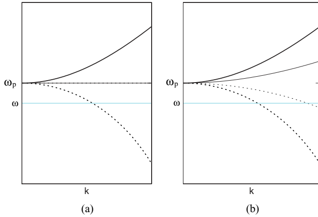
FIG. 2. (Color online) Dispersion relation for transverse waves (thick lines) and bulk plasmons (thin lines) when (a) the nonlocality is absent ( \beta = 0 ) and (b) the nonlocality is important. The dashed lines show the imaginary parts of the propagation constants for the transverse and longitudinal waves, below the plasma frequency \omega_p . When nonlocality is present, for a given \omega two waves must be taken into account.
