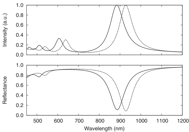
FIG. 11. Bottom: Reflection spectrum according to local (RCWA, dashed line) and nonlocal (COMSOL, solid line) simulations. Top: Model (54) for the field intensity under the strips for the local (dashed line) and nonlocal (solid line) theory. The agreement between the simulations and the model are in excellent agreement for the local as well as for the nonlocal theory.
